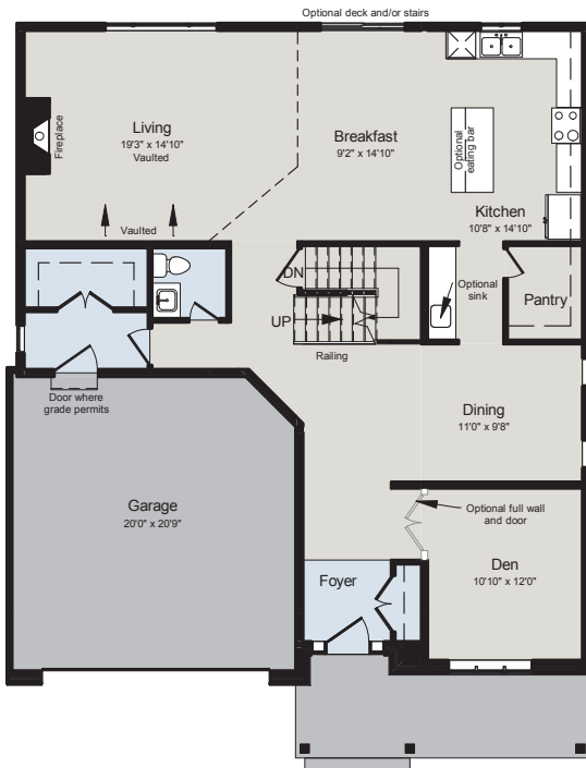
MAIN FLOOR
