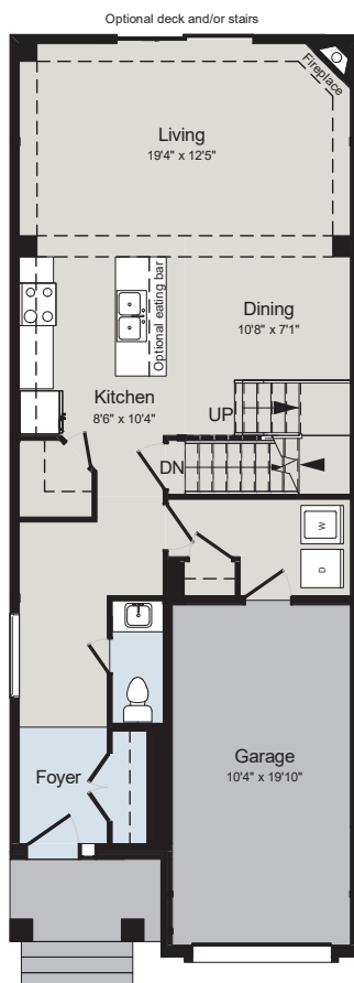
MAIN FLOOR
