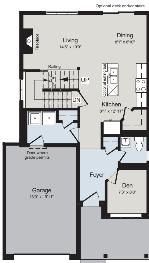
MAIN FLOOR
