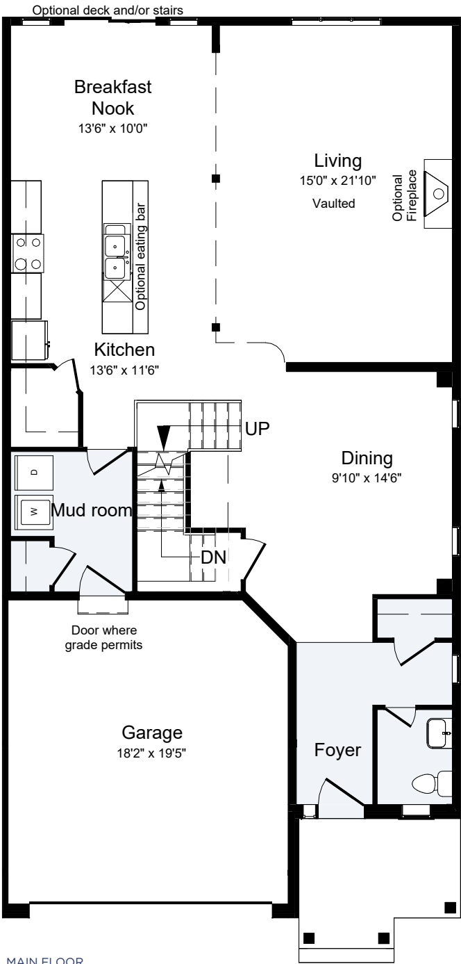
MAIN FLOOR
