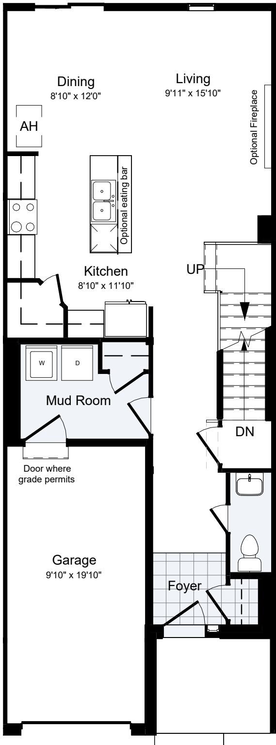
MAIN FLOOR
