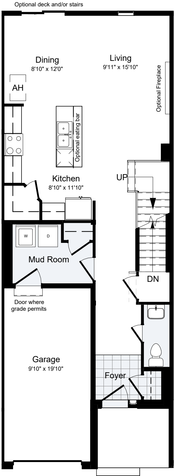
MAIN FLOOR
