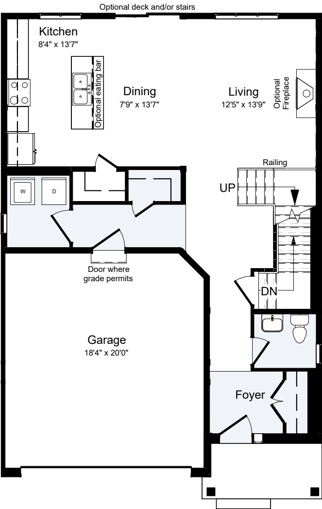
MAIN FLOOR
